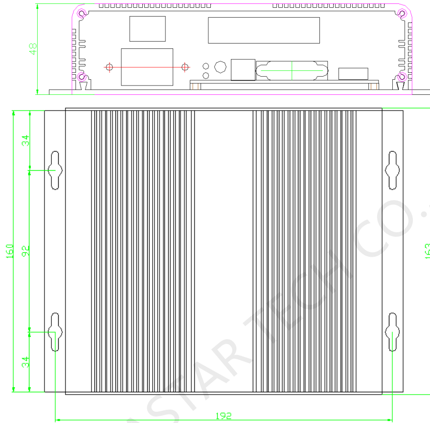
Fig. 1 MCTRL300 dimensions
